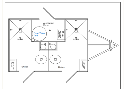
Floorplan · 2 Combo Stations
