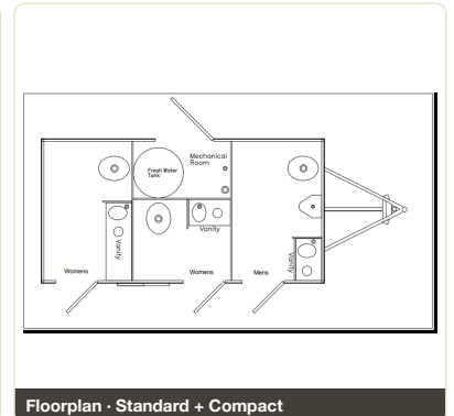
Floorplan · Standard + Compact
