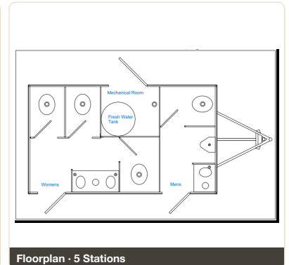
Floorplan · 5 Stations
