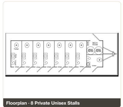
Floorplan · 8 Private Unisex Stalls
