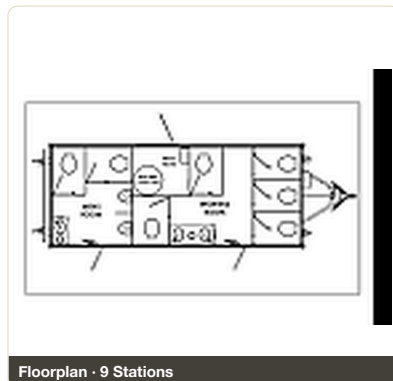
Floorplan · 9 Stations
